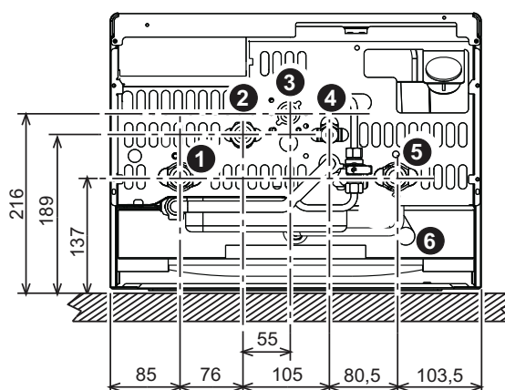
fig. 17 - Plumbing connections
