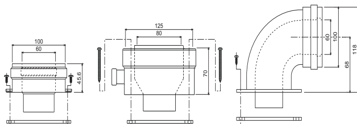
fig. 21 - Starting accessories for coaxial ducts
