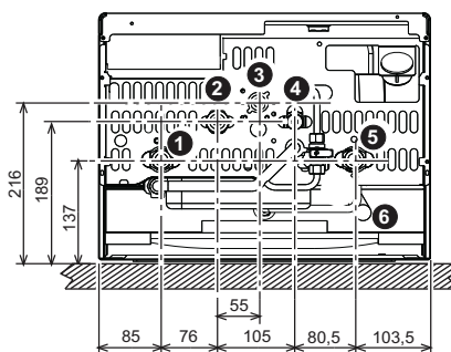
fig. 17 - Raccordements hydrauliques
