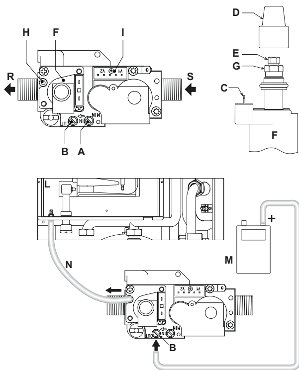
fig. 26 - Valvola gas
