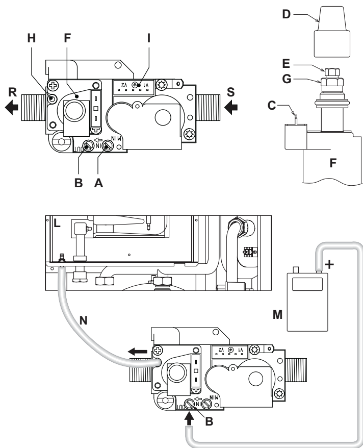
fig. 26 - Gas valve
