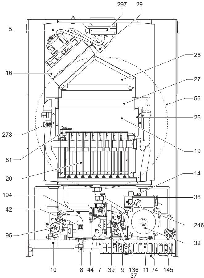
fig. 29 - Vista general DIVAtop MICRO LN F 24
