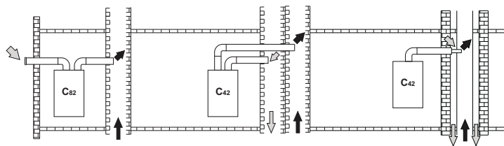
fig. 24 - Examples of connection to flues (⇨ = Air / ⇨ = Fumes)
