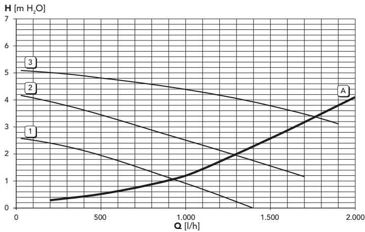
fig. 32 - Circulating pump head / pressure losses DIVAtop MICRO LN F 24
