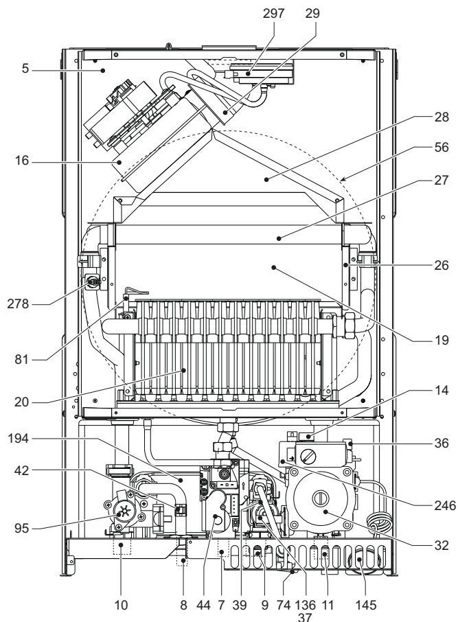
fig. 30 - General view DIVAtop MICRO LN F 32
