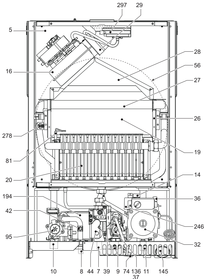
fig. 30 - Vista general DIVAtop MICRO LN F 32
