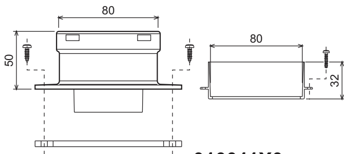
fig. 23 - Starting accessory for separate ducts
