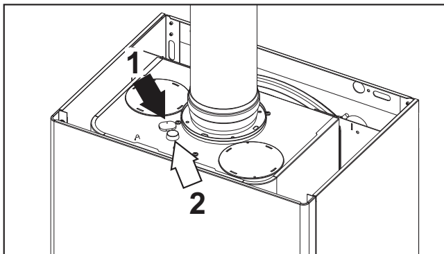
fig. 28 - Analizarea gazelor arse DIVAtop MICRO LN F 24
