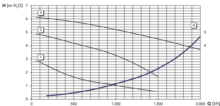
fig. 34 - Circulating pump head / pressure losses DIVAtop MICRO LN F 32
