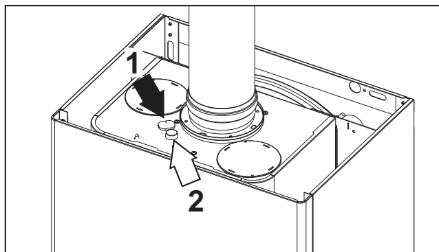
fig. 28 - Analisi fumi DIVAtop MICRO LN F 24
