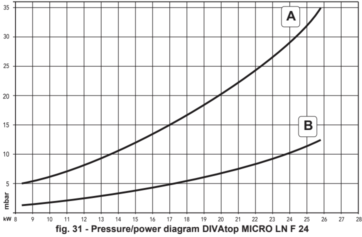
fig. 31 - Pressure/power diagram DIVAtop MICRO LN F 24
