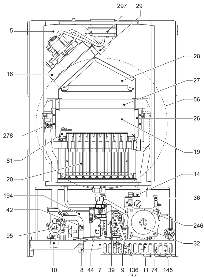
fig. 29 - General view DIVAtop MICRO LN F 24
