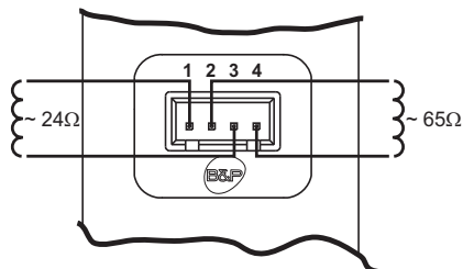
fig. 30 - Gas valve connection
